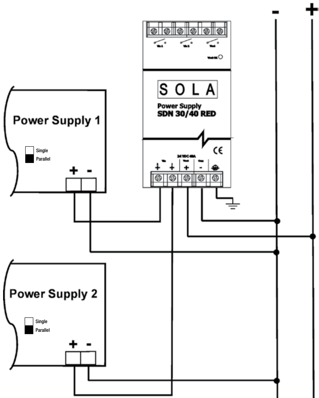
Wiring Diagram for SDN 30/40RED
